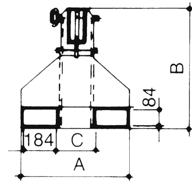
Fork Sleeve internal dimensions
